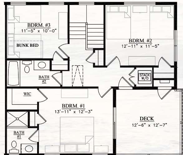
SECOND FLOOR
