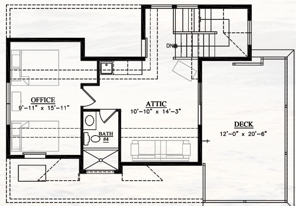
THIRD FLOOR / ATTIC
